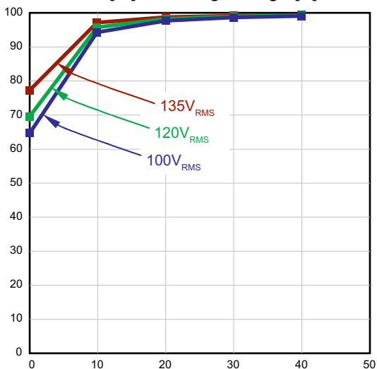
PF [%] vs. String Voltage [V]
